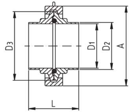
Clamp connection DIN 11853/3 11866 (B) Klemverbinding DIN 11853/3 11866 (B)
